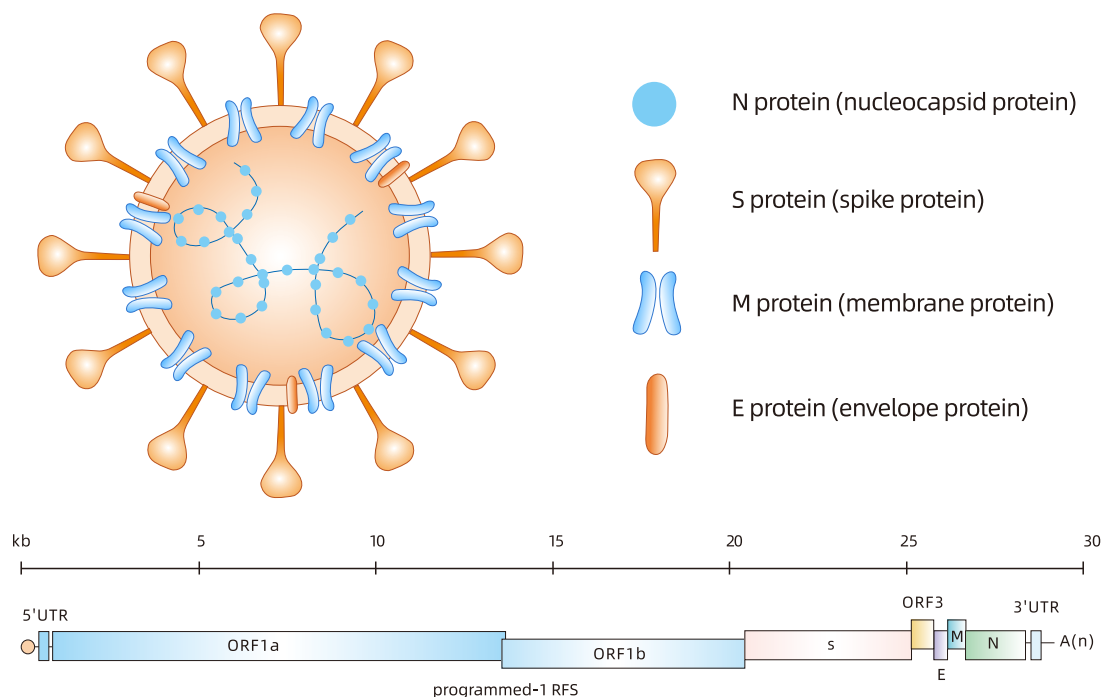
Fig.1 Schematic representation of PEDV genome organization and virion structure
